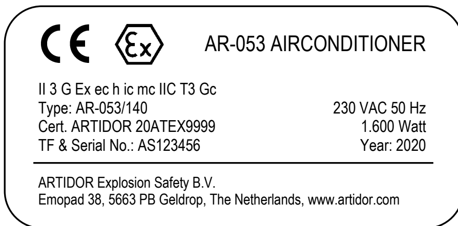
Example of an rooftop air conditioning unit label
